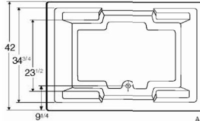
Tub pictured with optional grab bars and waste & overflow.
