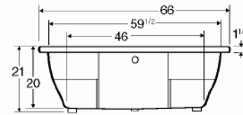
All bathtub dimensions are \pm 1/2'' .
